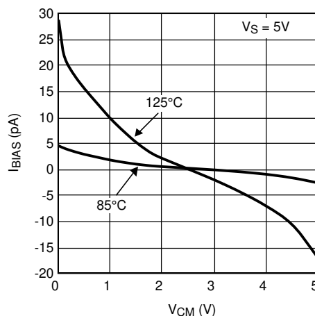
Figure 5-38. Input Bias Current vs Common Mode Voltage
