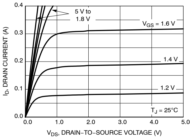
Figure 12. On-Region Characteristics
