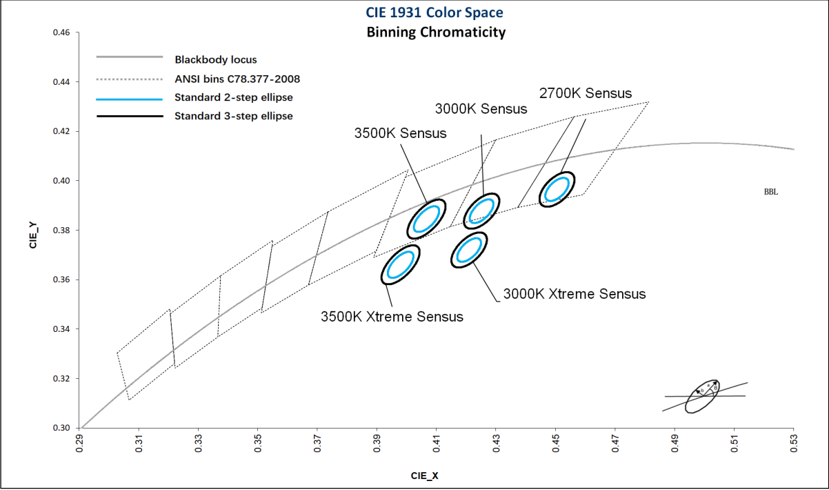
Chromaticity Binning Diagram 1 - TC62 Sensus and TC64 Xtreme Sensus (BBBL)
